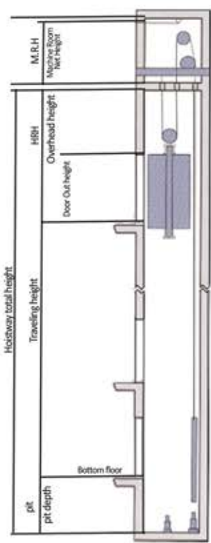
WITH MACHINE ROOM
