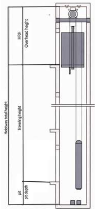
WITHOUT MACHINE ROOM
